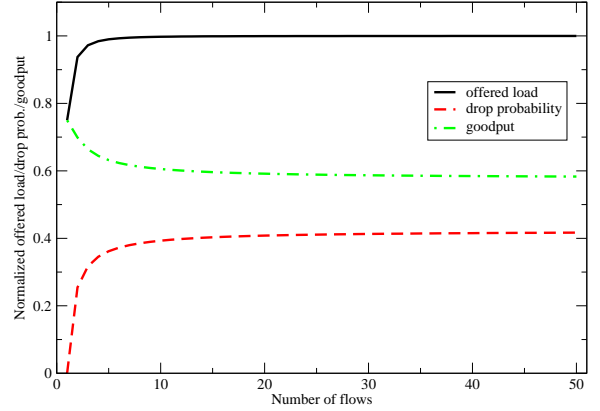
Fig. 3. The offered load (throughput), drop probability and the goodput at the Nash equilibrium imposed by EN-AQM as the number of flows passing through our router mechanism changes
