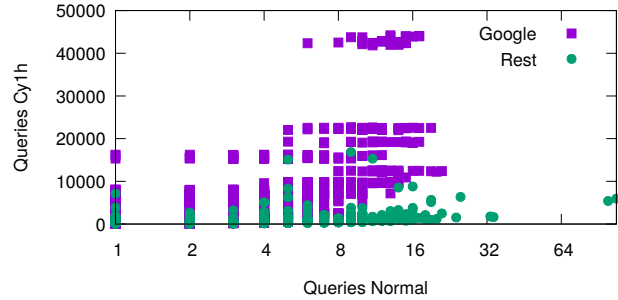
Figure 10: Resolvers with at least 100x traffic growth (A queries)
