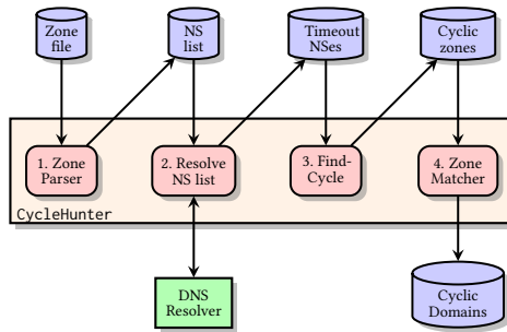
Figure 11: CycleHunter workflow
