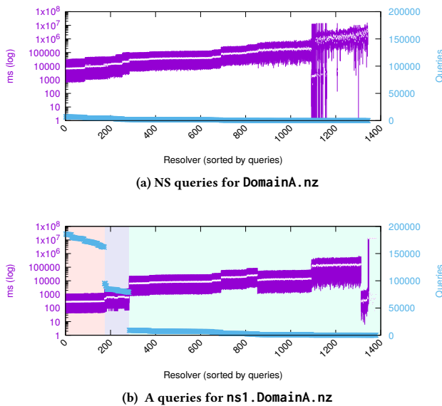
Figure 3: Google (AS15169) resolvers on 2020-02-06, during .nz TsuNAME event: time in between queries.
