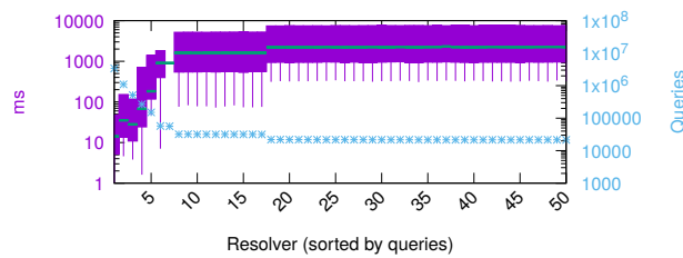
Figure 20: Recurrent: IQR and queries for A records of ns.vuur.cachetest.net
