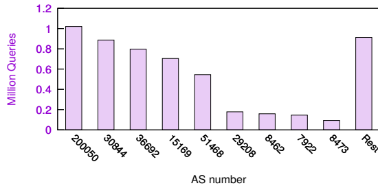
Figure 22: Top 10 ASes for TripleDep experiment
