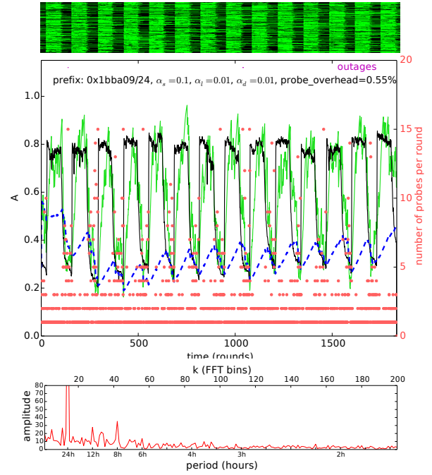
Figure 3: Block 27.186.9/24 from S_{51w} , |E(b)| = 256 , A = 0.598 . Diurnal block. Lines described in Figure 1. Bottom: amplitude of FFT ( N_d = 14 ) of \hat{A}_s showing strong diurnal amplitude.
