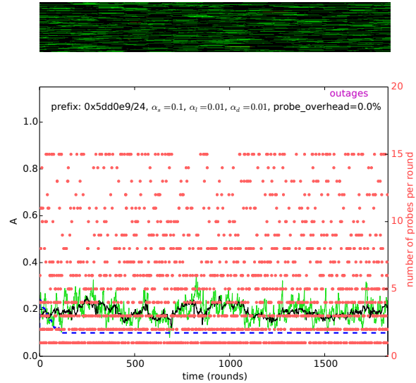
Figure 2: Block 93.208.233/24 from S_{51w} , |E(b)| = 245 , A = 0.191 . Dense but low availability block. (Block is non-diurnal, so FFT is omitted.) Lines described in Figure 1.
