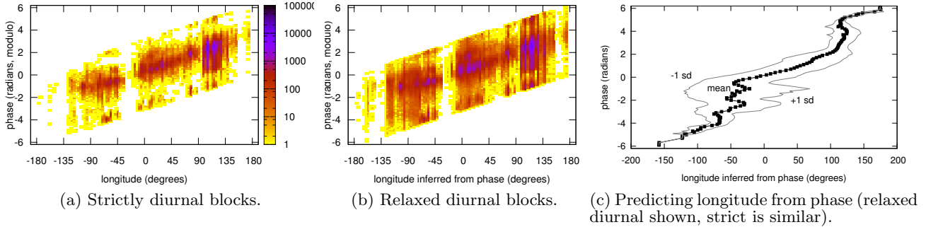
Figure 14: Comparing phase and longitude. Dataset: A_{12w} .
