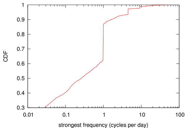
Figure 10: Cumulative distribution of the highest frequency in 35-day A_{12w} .
