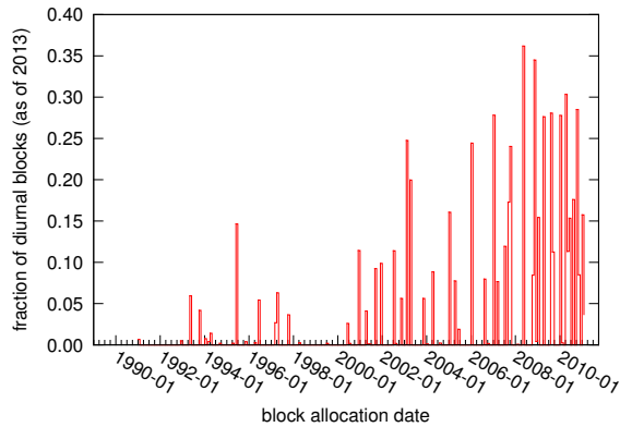
Figure 15: Percentage of diurnal blocks in each month, based on block allocation date. Dataset: 2013 diurnalness: A_{12w} ; block allocation: IANA).
