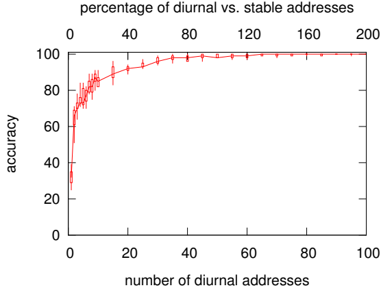
Figure 7: Accuracy of diurnal detection when the number of diurnal behavior addresses ( n_d ) per block varies from 2% to 67% of responsive addresses ( \Phi = \sigma_s = \sigma_d = 0 ). Data: simulation.
