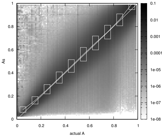
Figure 4: Correlation of actual ( A ) and estimated ( \hat{A}_s ) availability. Density is normalized by the product of number of blocks and rounds. Quartiles show A_s , binned by 0.1A .
