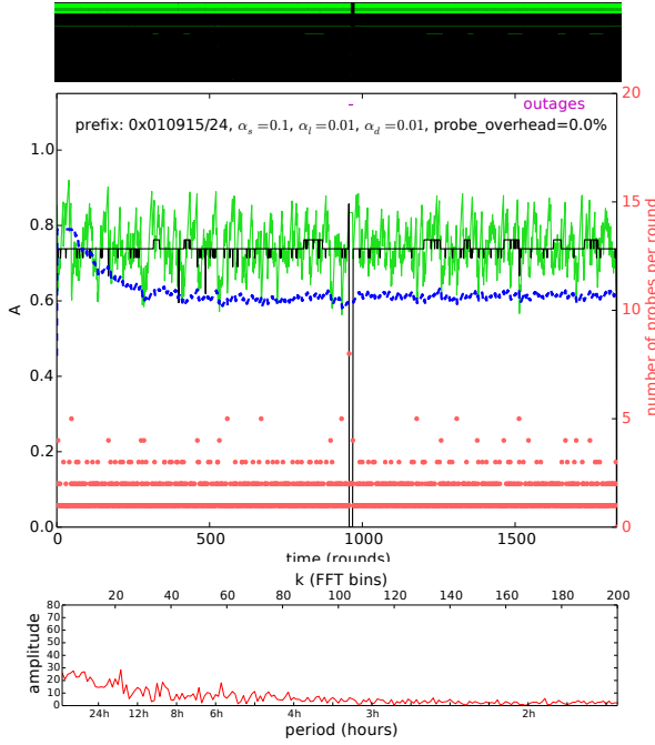
Figure 1: Block 1.9.21/24 from S_{51w} , a sparse but high availability block (42 every responding addresses, A = 0.735 ). Top: raw survey data: green is response, black is no response. Middle: compares true A (black, upper line with minimal variation), short-term estimate \hat{A}_s (light green, upper line with larger variation), operational estimate \hat{A}_o (dotted dark blue, lower line), and report the number probes per round (red dots at bottom and right scale). An outage occurs at round 957 (the magenta line). Probes-per-round (red dots, mostly along the bottom) use the right scale. Bottom: amplitude of FFT ( N_d = 14 ) of \hat{A}_s , with no strong diurnal signals.
