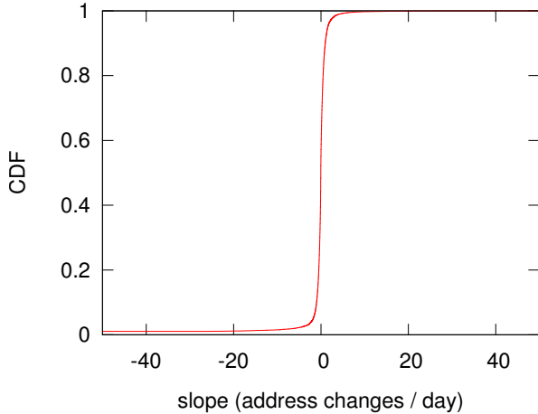
Figure 18: Checking stationarity of all blocks in Survey S_{51w} , showing the slope of linear regression on true availability A .
