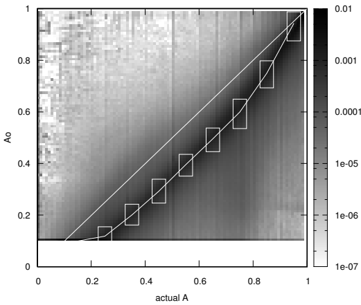
Figure 5: Correlation of actual ( A ) and operational ( \hat{A}_o ) availability. Density is normalized by the product of number of blocks and rounds. Quartiles show A_o , binned by 0.1A .
